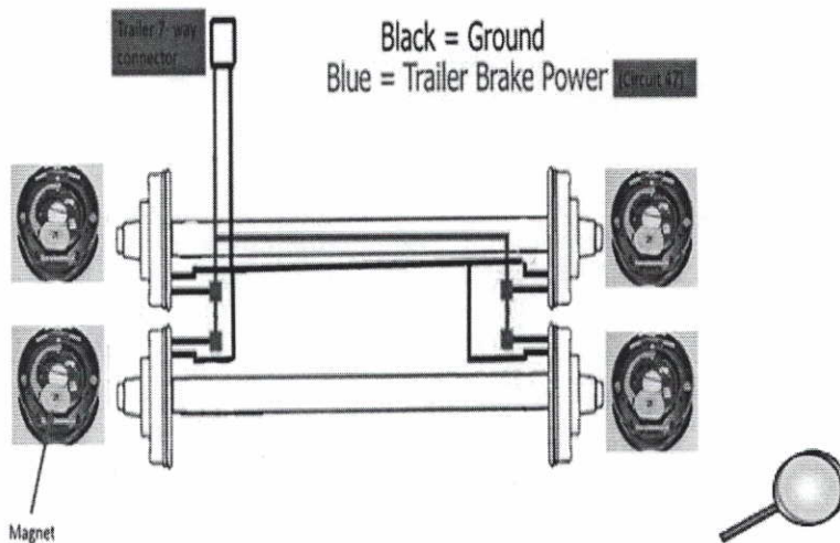
Example of a 2 axle trailer with electric trailer brakes
