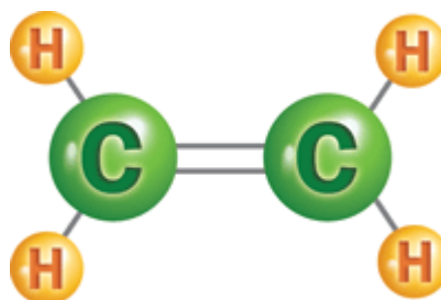
Alpha-olefin molecule
