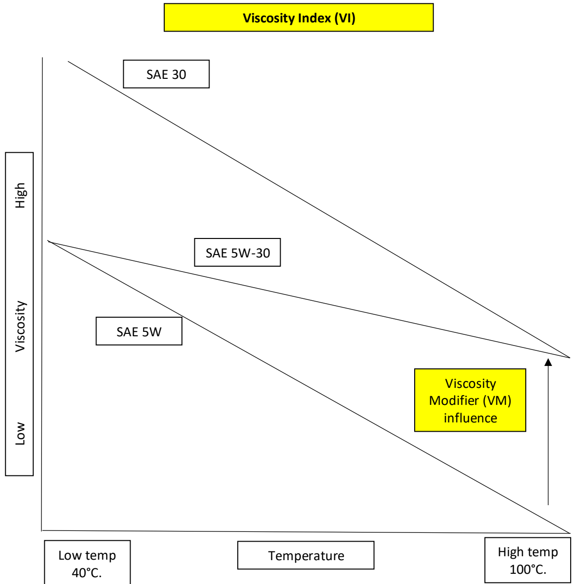
How the Viscosity Modifier (VM) responds to changes in oil temperature
