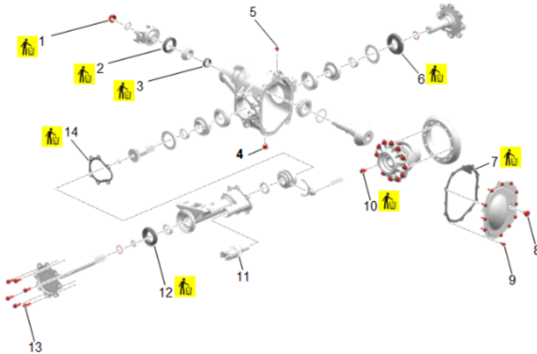
Front Differential Carrier and Components
