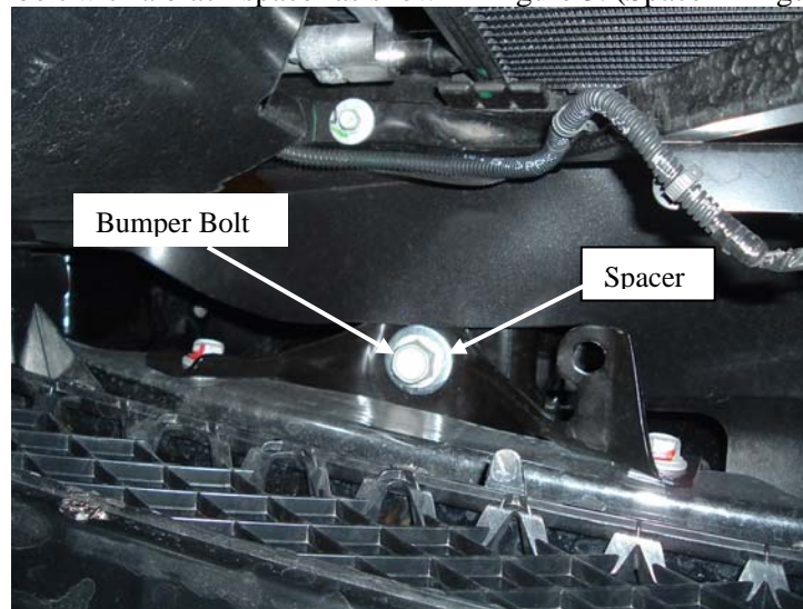
Figure 5. Bumper Bolt and spacer
