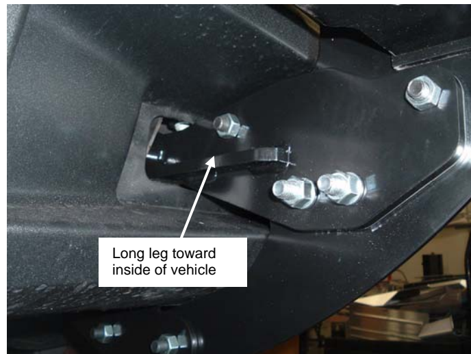
Figure 4 Frame Extension Installed
